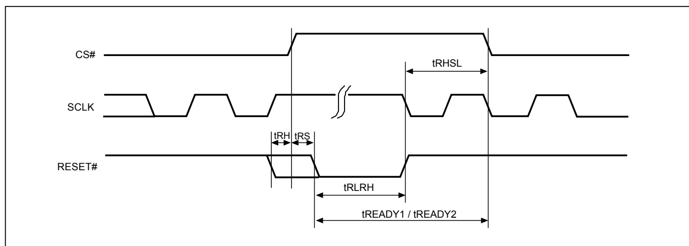
Figure 101. RESET Timing
