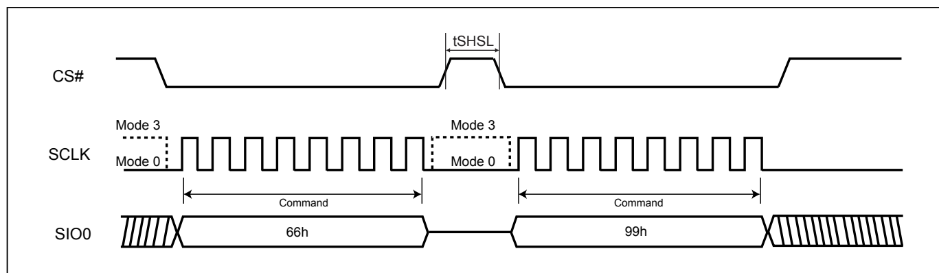
Figure 38. Reset Sequence
