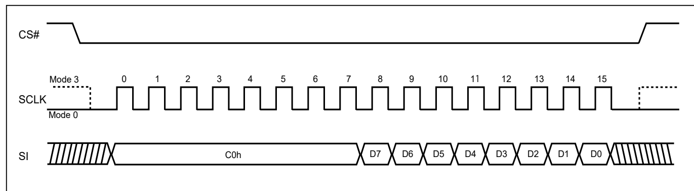
Figure 23. Burst Read
