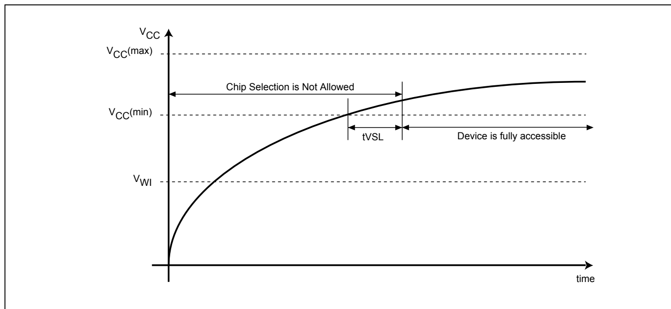
Figure 48. Power-up Timing
