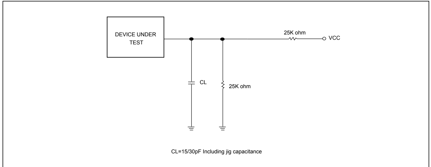
Figure 45. Output Loading
