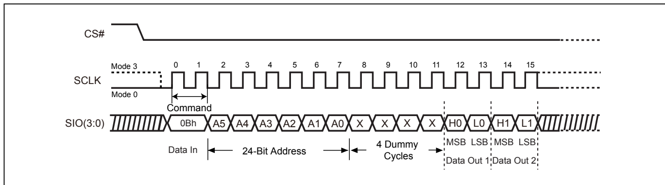
Figure 36. Read at Higher Speed (FAST_READ) Sequence (QPI Mode)
