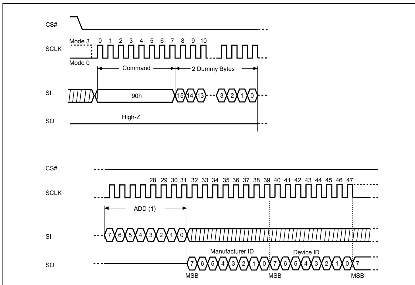
Figure 24. Read Electronic Manufacturer & Device ID (REMS) Sequence (SPI Mode only)
