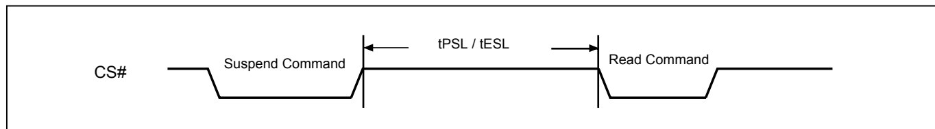
Figure 94. Suspend to Read Latency
