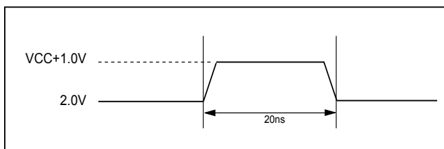
Figure 103. Maximum Positive Overshoot Waveform
