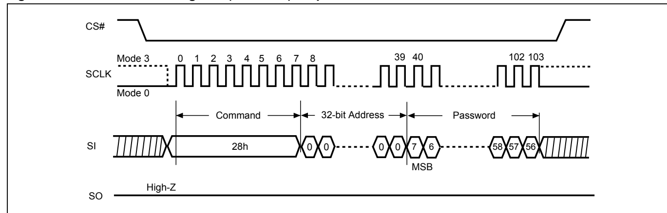
Figure 92. Write Password Register (WRPASS) Sequence
