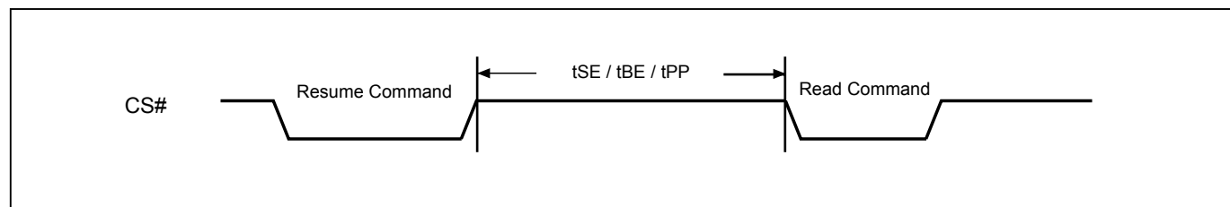
Figure 95. Resume to Read Latency
