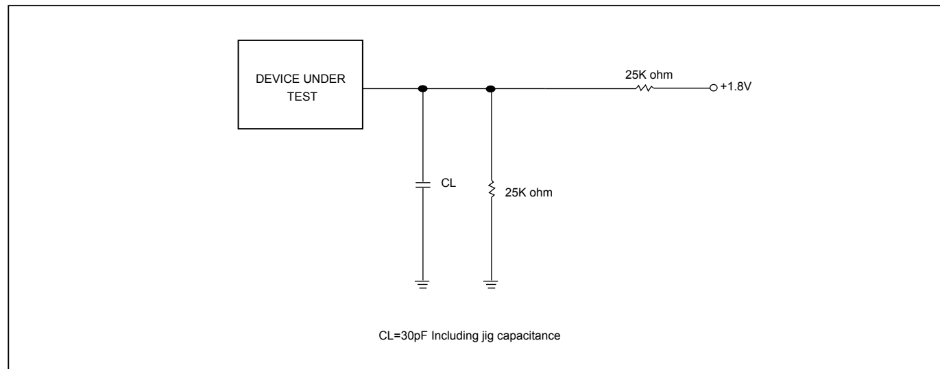
Figure 105. OUTPUT LOADING
