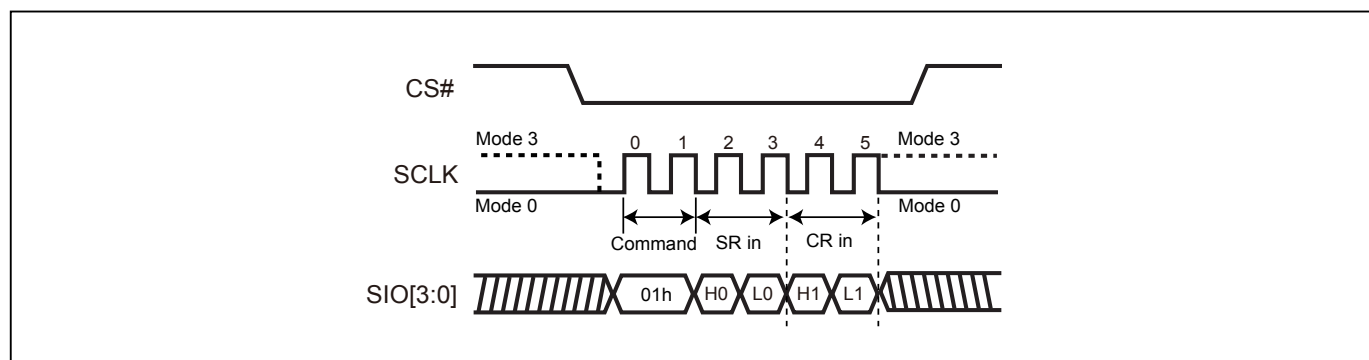
Figure 30. Write Status Register (WRSR) Sequence (QPI Mode)
