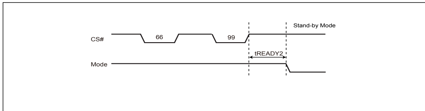
Figure 97. Software Reset Recovery
