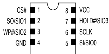
Figure 2. 8-WSON (8x6mm), 8-WLGA (6x5mm)
