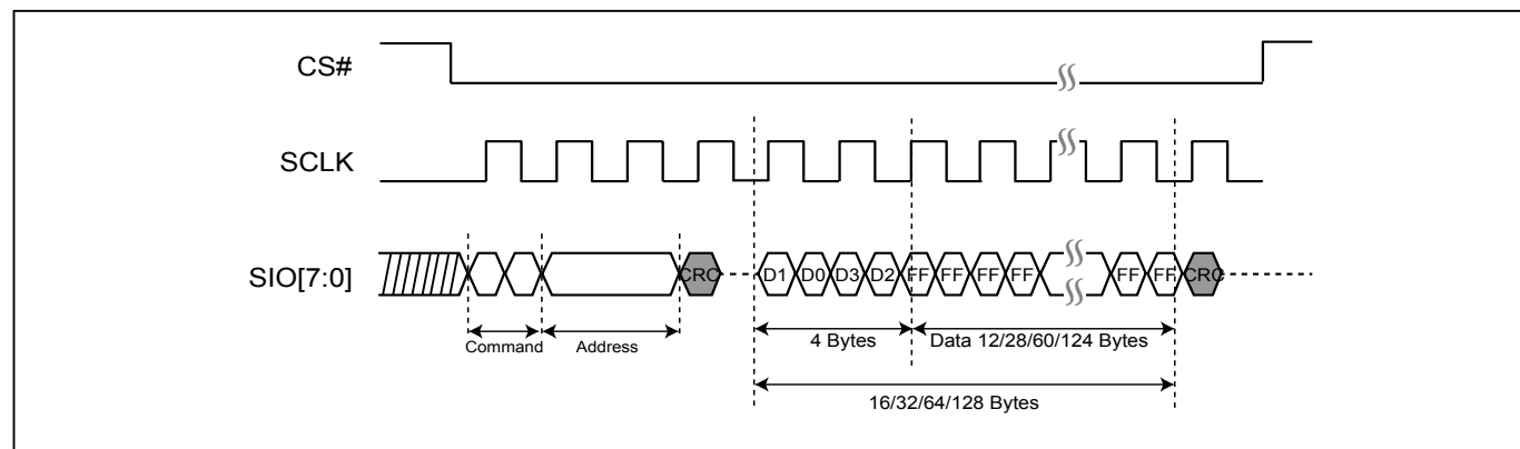
Figure 125. CRC Timing (WRFBR)
