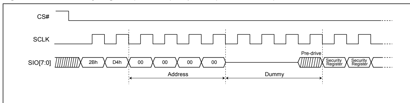
Figure 35. Read Security Register (RDSCUR) Sequence (STR-OPI Mode)
