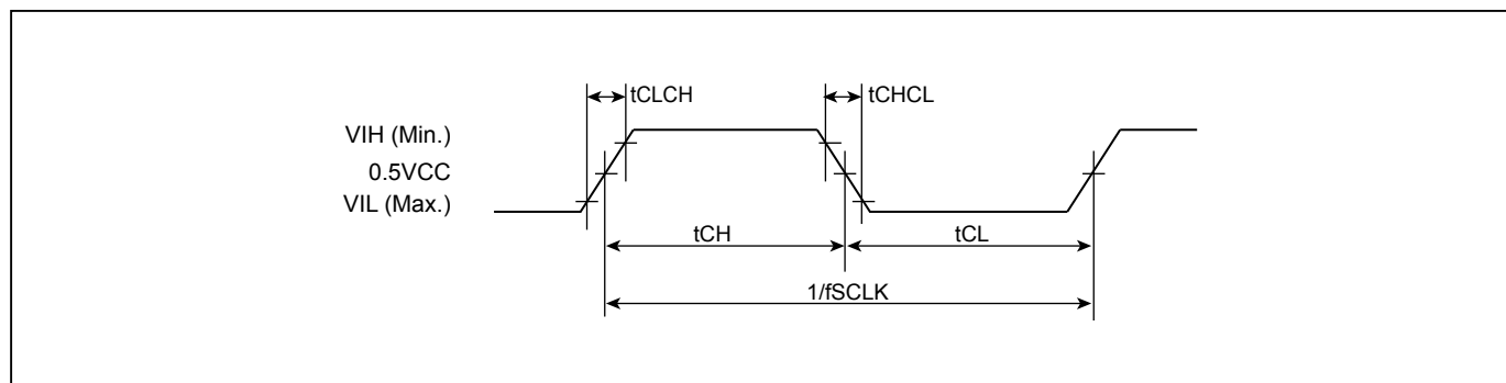
Figure 130. SCLK TIMING DEFINITION
