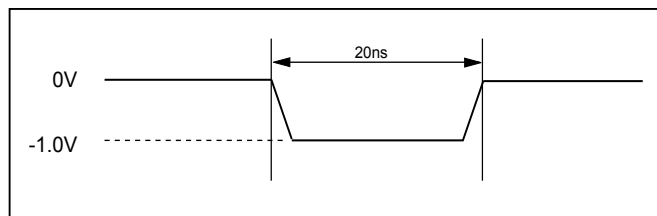
Figure 127. Maximum Negative Overshoot Waveform
