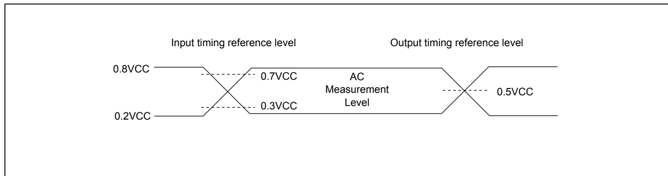
Figure 129. DATA INPUT TEST WAVEFORMS AND MEASUREMENT LEVEL
