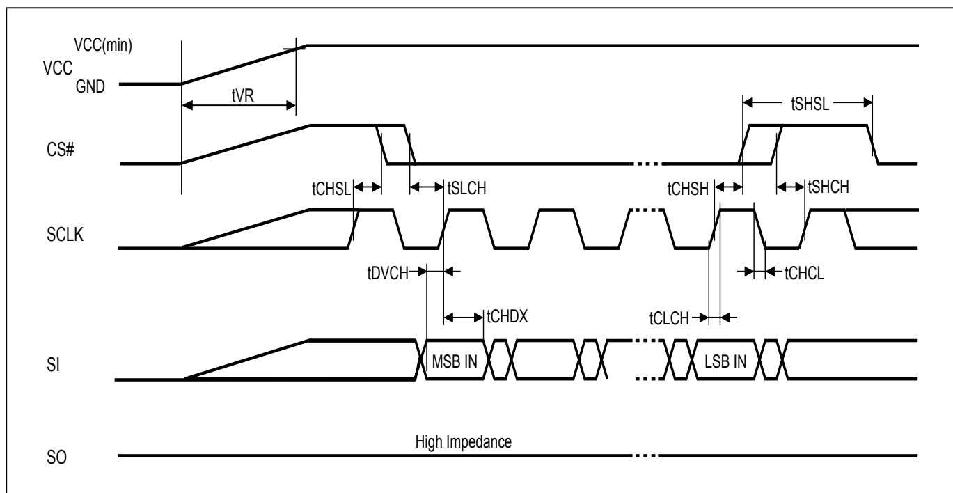
Figure 131. AC Timing at Device Power-Up
