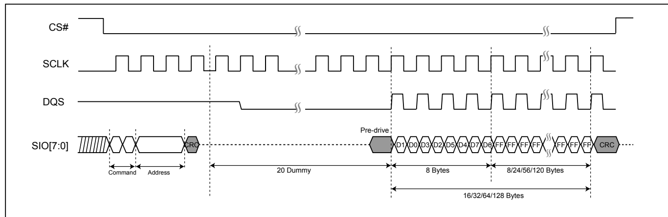
Figure 123. CRC Timing (RDPASS)
