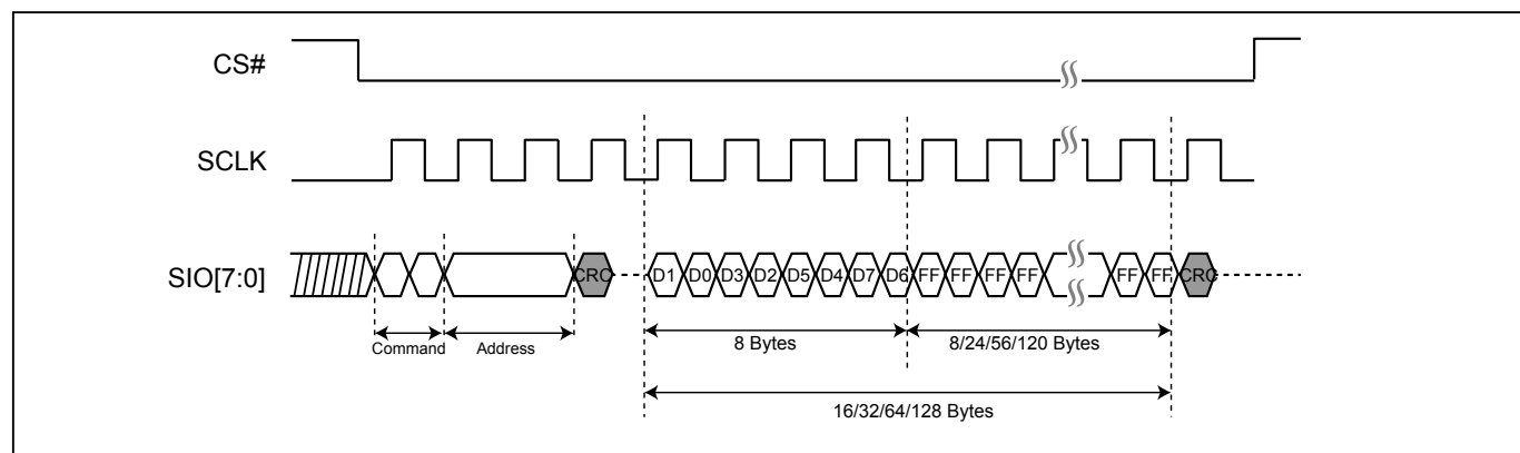
Figure 124. CRC Timing (WRPASS/PASSULK)
