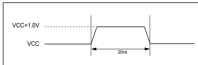
Figure 128. Maximum Positive Overshoot Waveform
