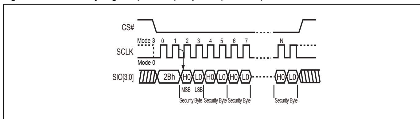
Figure 71. Read Security Register (RDSCUR) Sequence (QPI Mode)
