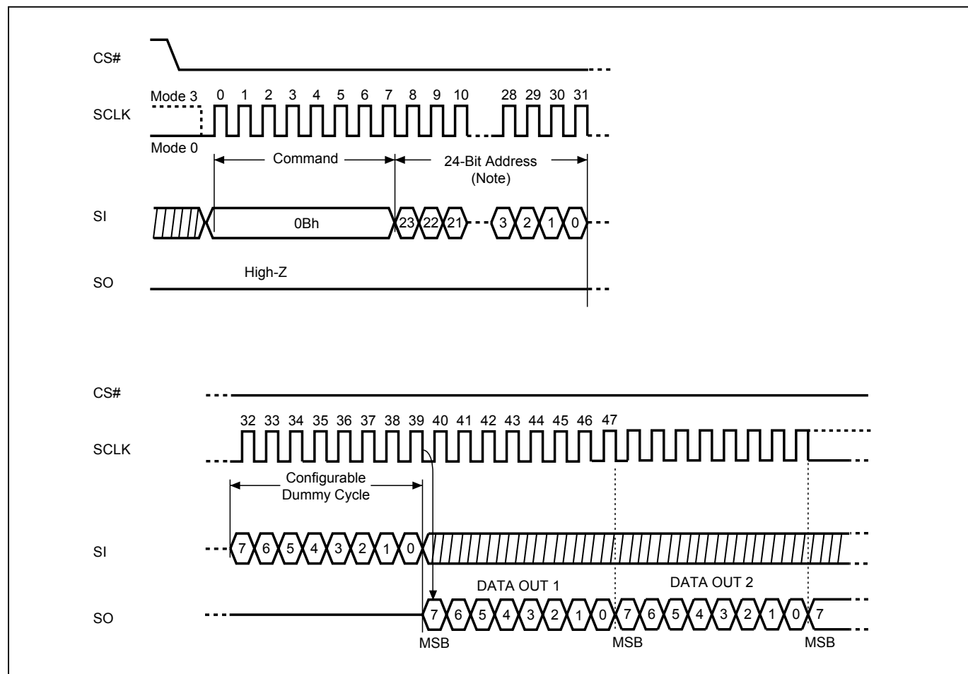
Figure 32. Read at Higher Speed (FAST_READ) Sequence (SPI Mode only)
