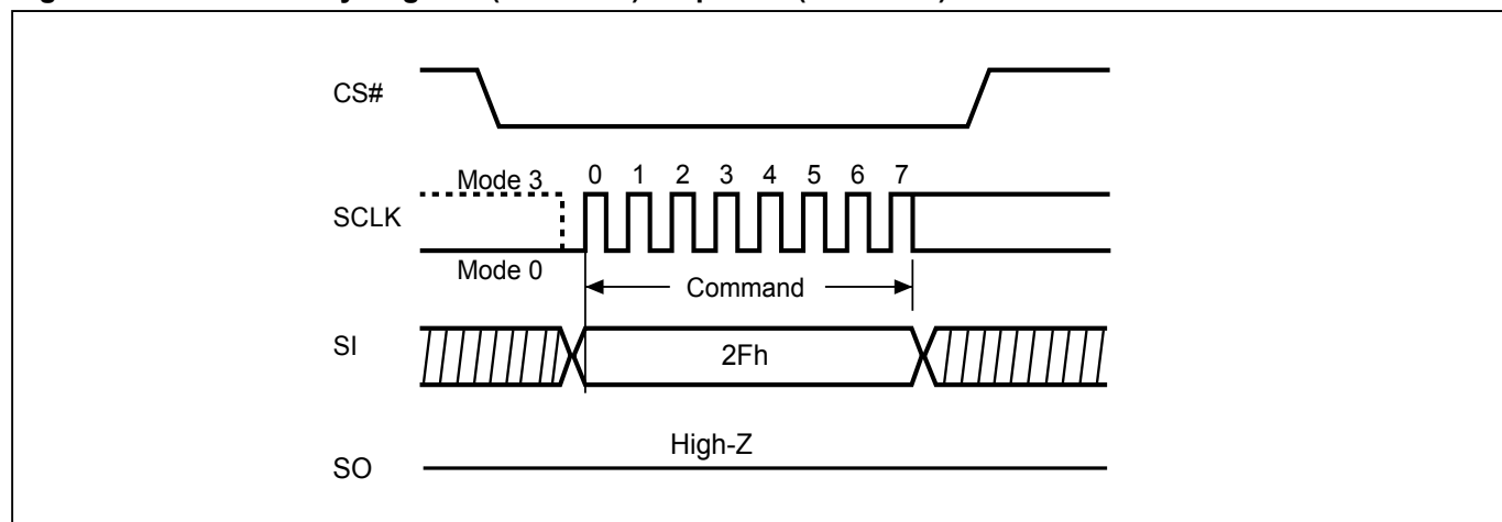
Figure 72. Write Security Register (WRSCUR) Sequence (SPI Mode)
