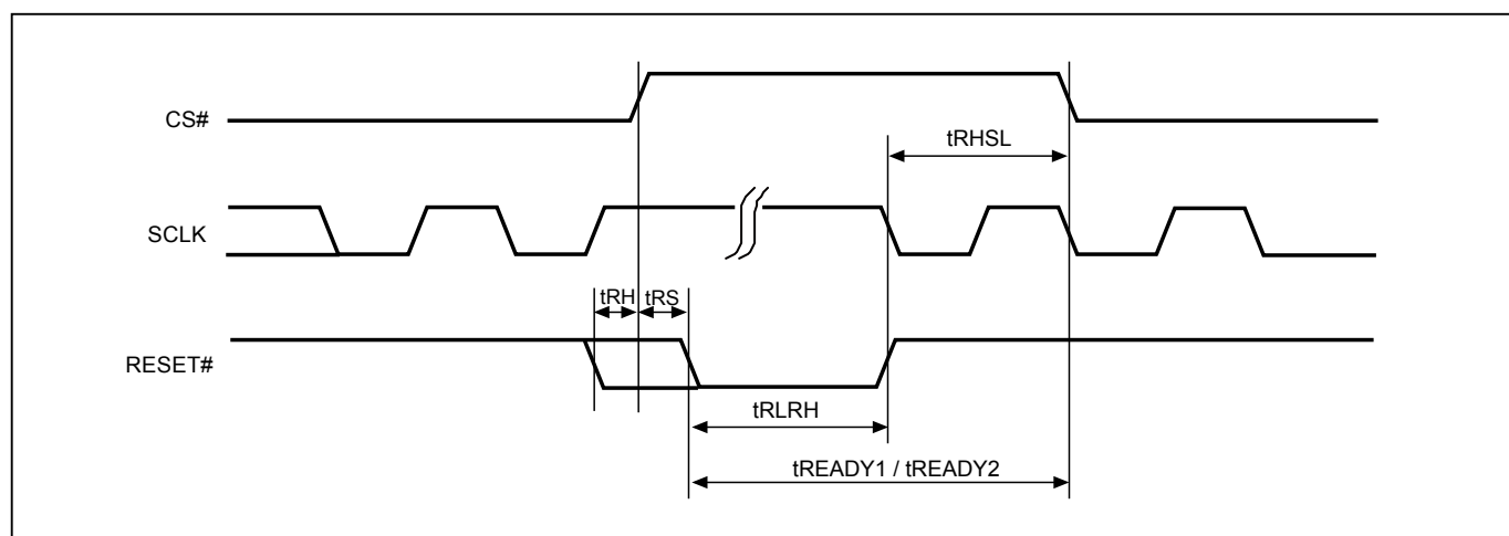
Figure 91. RESET Timing
