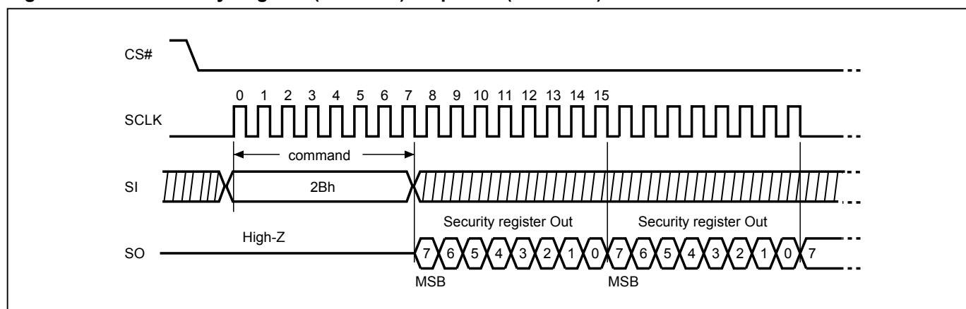
Figure 70. Read Security Register (RDSCUR) Sequence (SPI Mode)
