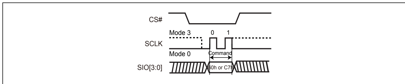
Figure 55. Chip Erase (CE) Sequence (QPI Mode)
