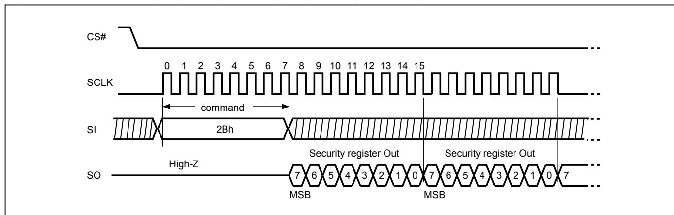
Figure 63. Read Security Register (RDSCUR) Sequence (SPI Mode)
