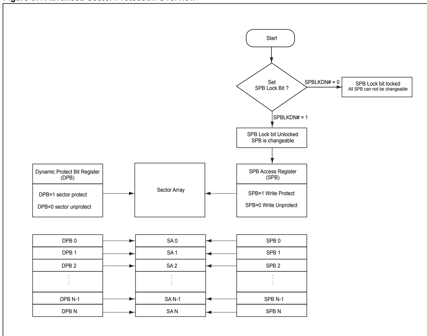
Figure 67. Advanced Sector Protection Overview
