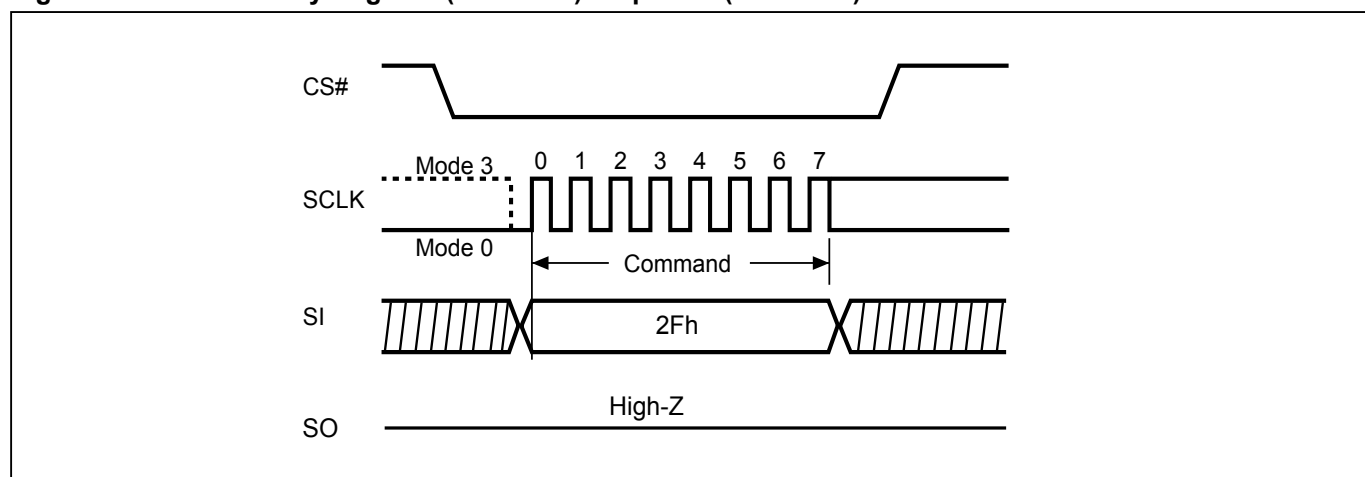
Figure 61. Write Security Register (WRSCUR) Sequence (SPI Mode)
