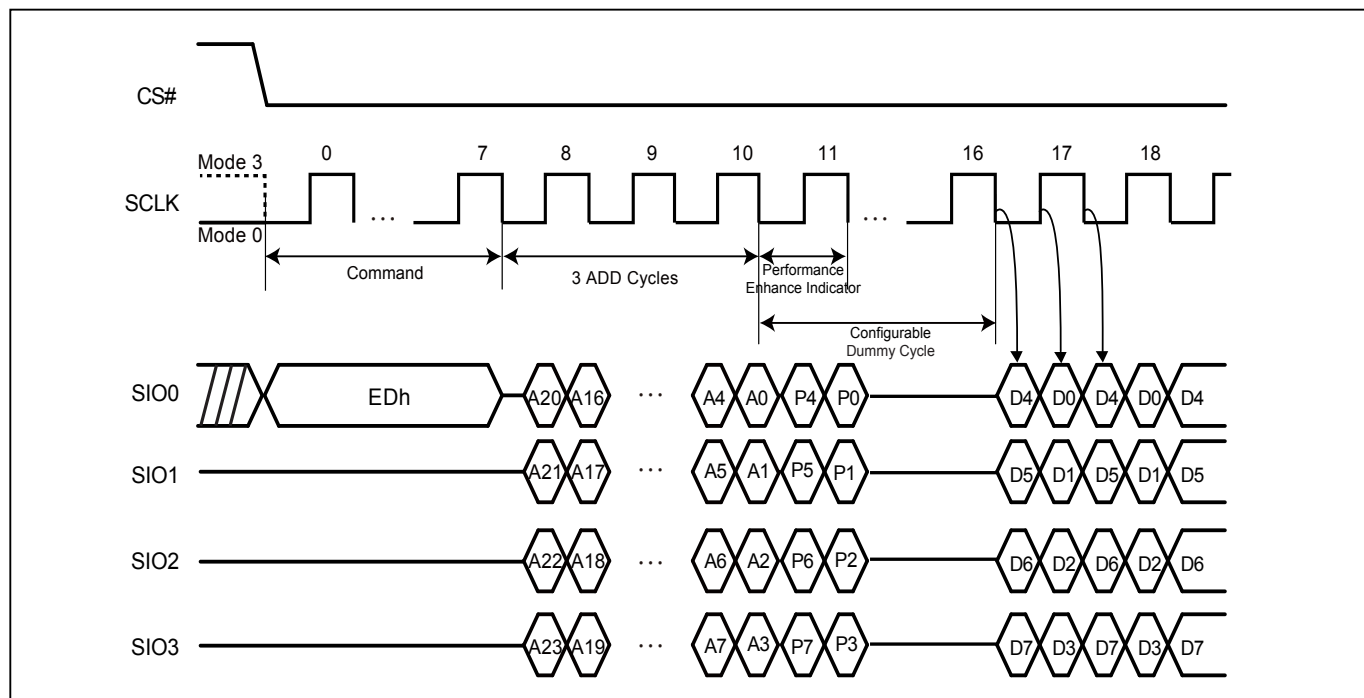
Figure 35. Fast Quad I/O DT Read (4DTRD) Sequence (SPI Mode)
