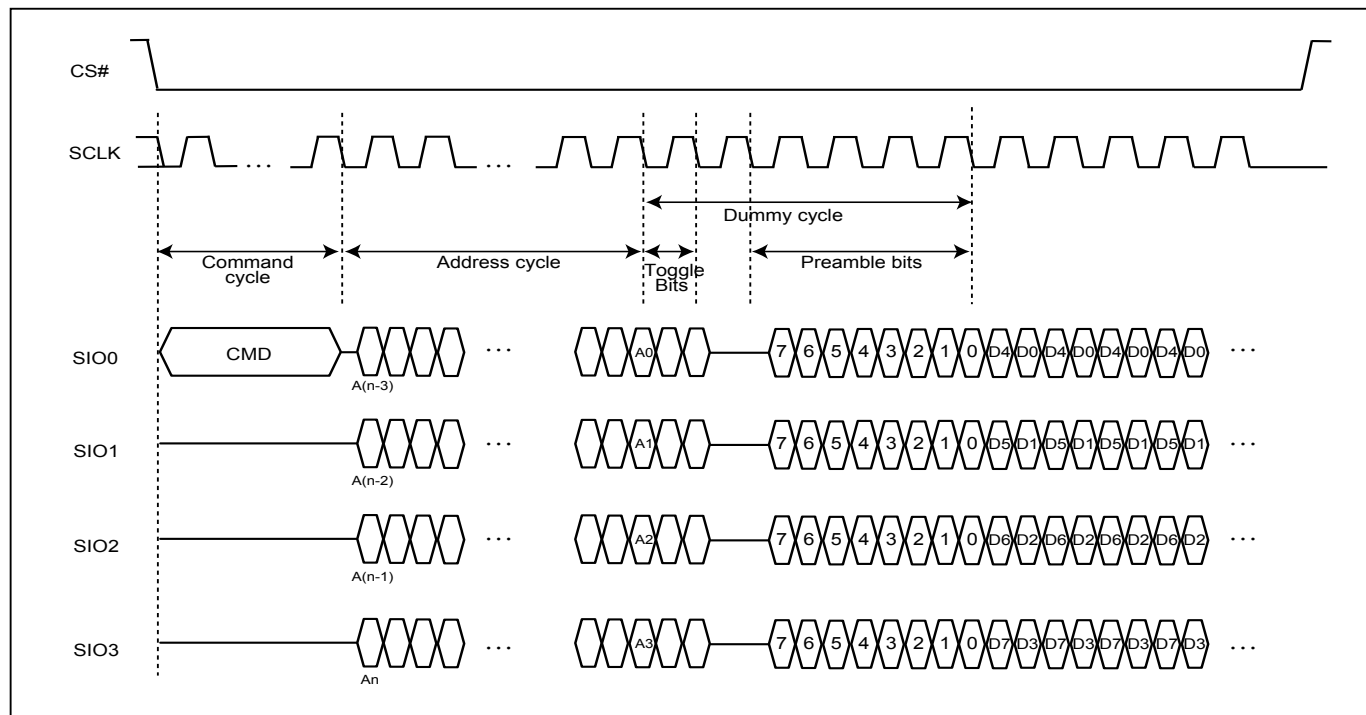
Figure 43. DTR4IO (6DC)
