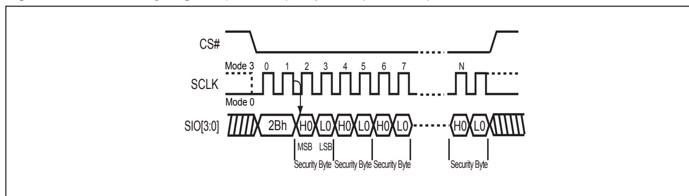
Figure 64. Read Security Register (RDSCUR) Sequence (QPI Mode)
