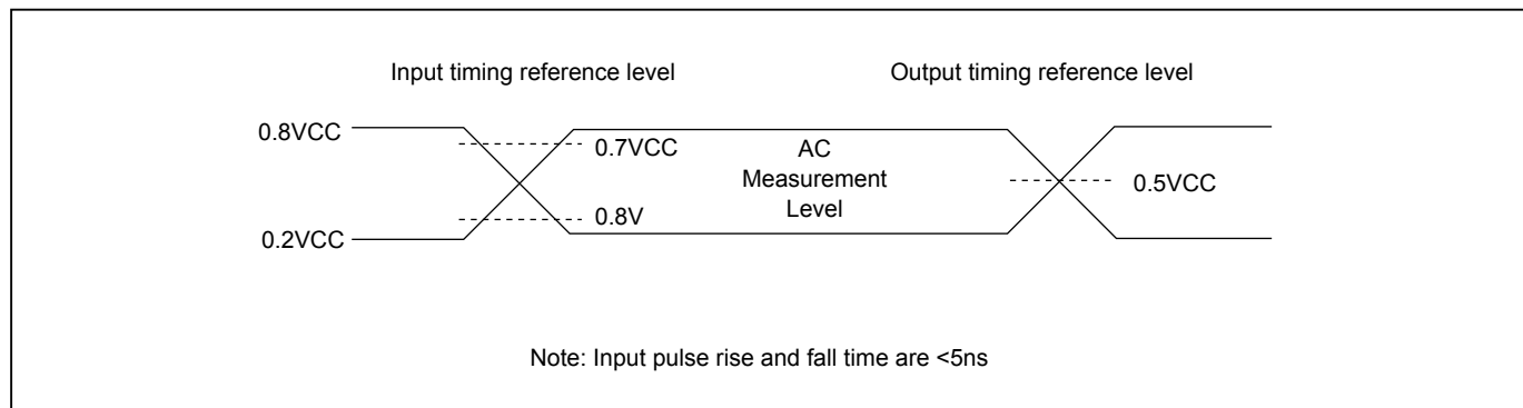
Figure 85. DATA INPUT TEST WAVEFORMS AND MEASUREMENT LEVEL
