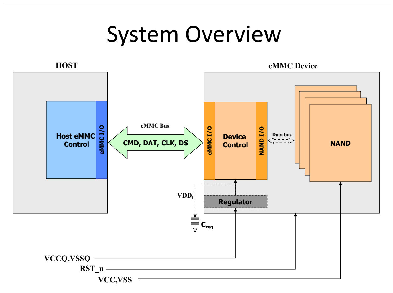
Figure 1. Logic Diagram
