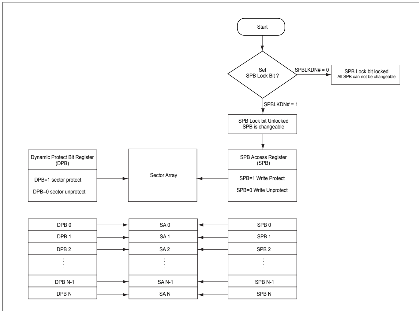
Figure 55. Advanced Sector Protection Overview
