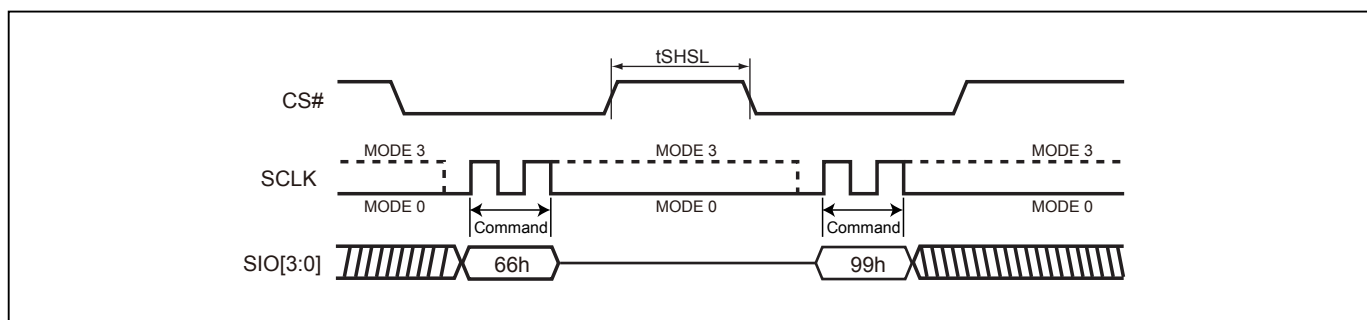
Figure 68. Reset Sequence (QPI mode)
