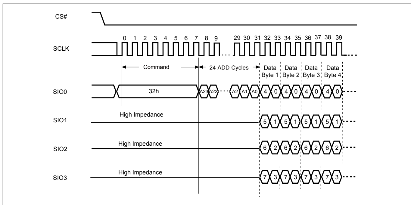
Figure 50. Quad Input Page Program (QPP) Sequence
